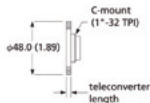
HE15-1/2XE teleconverters for C-mount lenses
