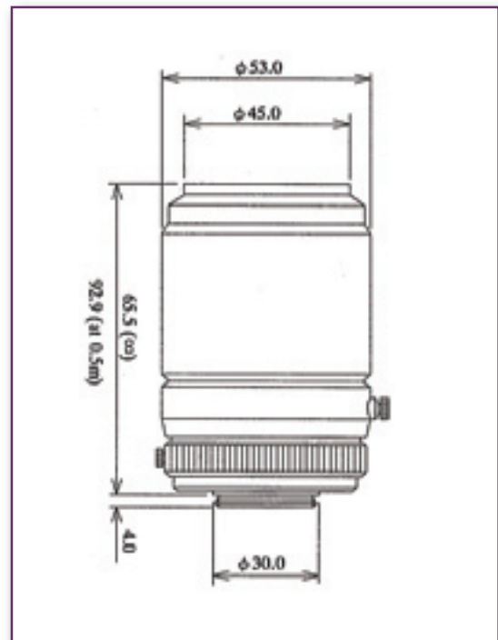
TEC-55 Outline Drawing with Dimensions
