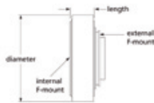
59 LGZ 814/820 teleconverters for F-mount lenses
